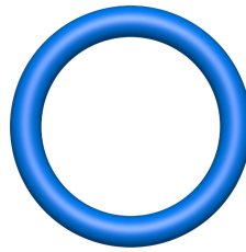
FIGURE 4.3: The unknot
